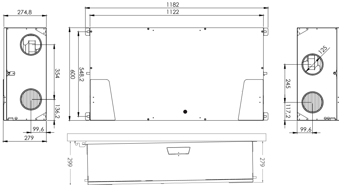
Illustration of duct connections in fan direction mode A:
